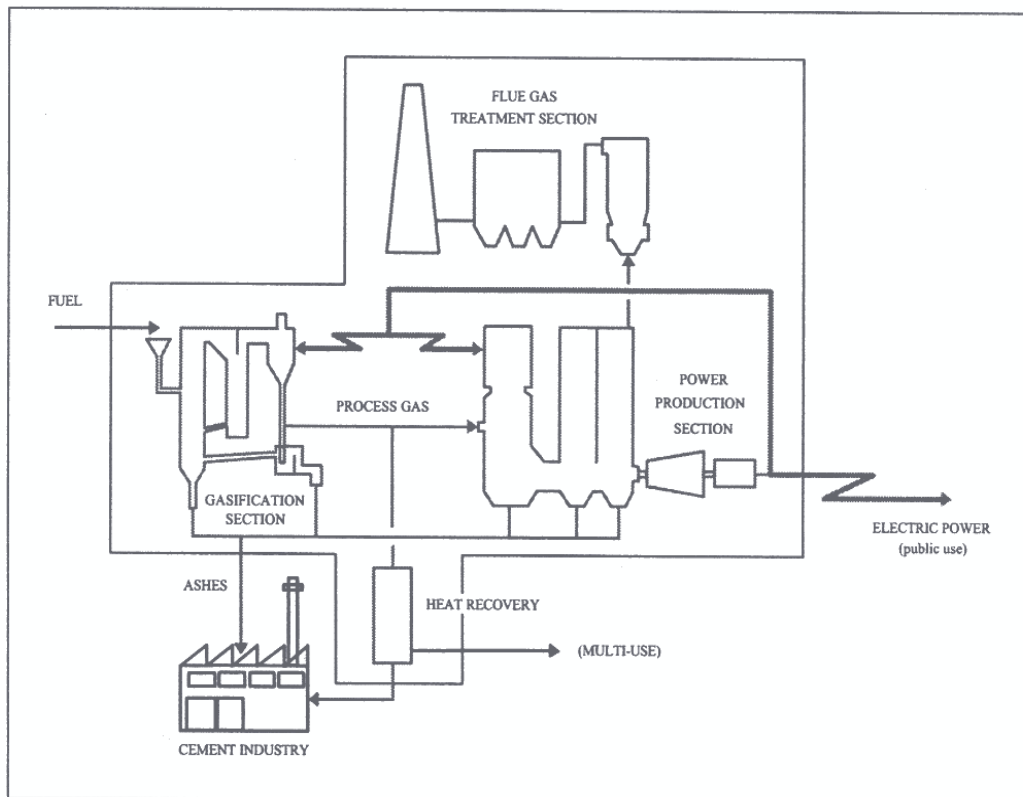
Figure 2. Process Scheme of Greve in Chianti RDF Gasification Plant, Italy
