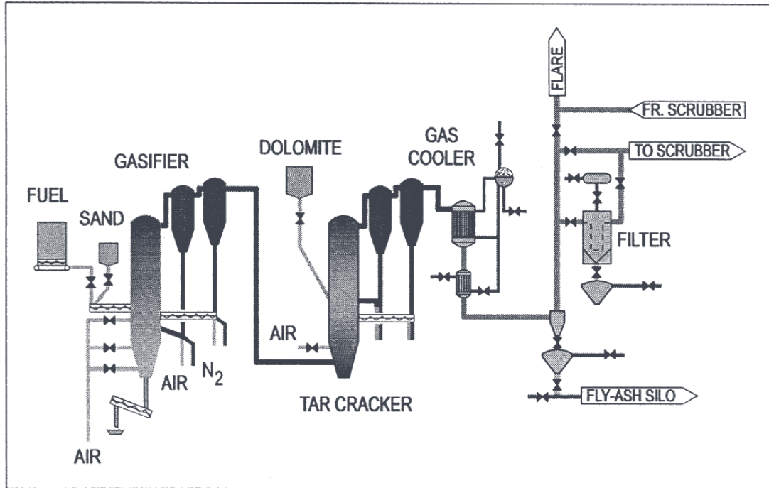
Figure 1. Termiska Processor (TPS) CFB Gasification Pilot Plant
